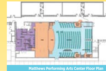
Mattheus Performing Arts Center Floor Plan
